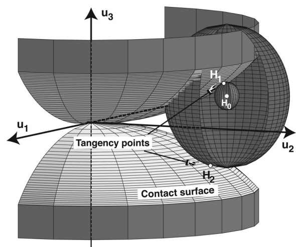
Fig. 4. The contact surface in \mathbf{u} -space is obtained by rotating the curve in Fig. 3A around the vertical axis. Given an unstressed configuration in the forbidden region (due to self-penetration) represented by a point H_0 , there exist two helices with self-contact and no external loading obtained by finding the tangency points of the contact surface with a level set of the energy W_1 = C in the upper (right-handed) and lower (left-handed), half space. The two tangency points correspond to the solutions H_{1,2} of Fig. 3.
