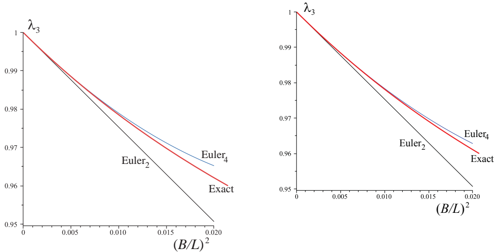
Figure 2: Comparison of the different Euler formulas obtained by expanding the exact solution to order 2 (classical Euler buckling formula, plot labeled “Euler 2 ”) and to order 4 (plot labeled “Euler 4 ”), for pyrex (figure on the left) and for silica (figure on the right).
