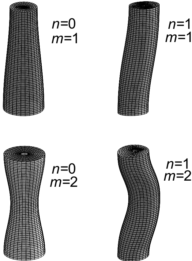
Figure 1: First two axi-symmetric and two asymmetric modes of buckling for a compressed strut with guided-guided end conditions: n is the circumferential mode number and m the axial mode number. For slender enough cylinders, the n = 1, m = 1 mode is the first mode of buckling.
