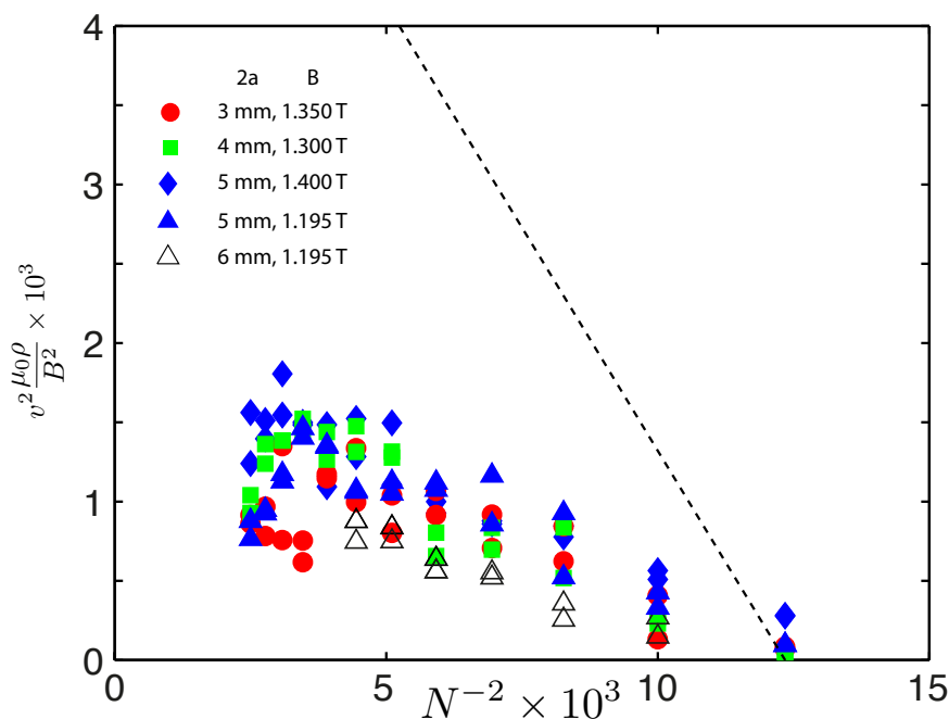
Figure 8. Rescaled square of the terminal velocity of a self-assembling cylinder as a function of N^{-2} . As described in the text, the squared velocity scales linearly with N^{-2} . The dotted line is the theoretical prediction (4.8) with the pre factor \alpha modified by the efficiency \mathcal{E} (see main text). The symbols used to encode different sphere sizes and magnetizations are as described in the legend.
