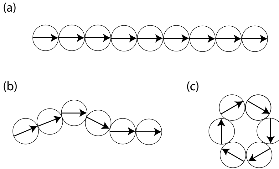
Figure 3. The physical mechanism behind the resistance to deformation of a magnetic chain. (a) In a straight chain all of the magnetic dipoles are aligned. (b) When deformed the dipoles can no longer be aligned. This frustration gives rise to a torque that resists deformation. (c) The general problem of determining the dipole orientation for a given deformation is in principle complicated [11]; here we consider a model calculation based on computing the energy required to form closed rings from chains.
