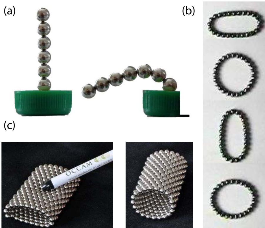
Figure 2. Three simple experiments that illustrate the resistance to deformation of assemblies of ferromagnetic spheres. (a) The self-buckling of a vertical chain of magnetic spheres as further spheres are added. (b) The prolate-oblate oscillation of a ring of magnetic spheres. Snap-shots of the motion are shown at intervals of 0.021 s. (c) A self-assembled chiral 'nano-tube'. In each case, the diameter of the spheres is 2a = 5 mm and the magnetic field strength is B = 1.195 T.
