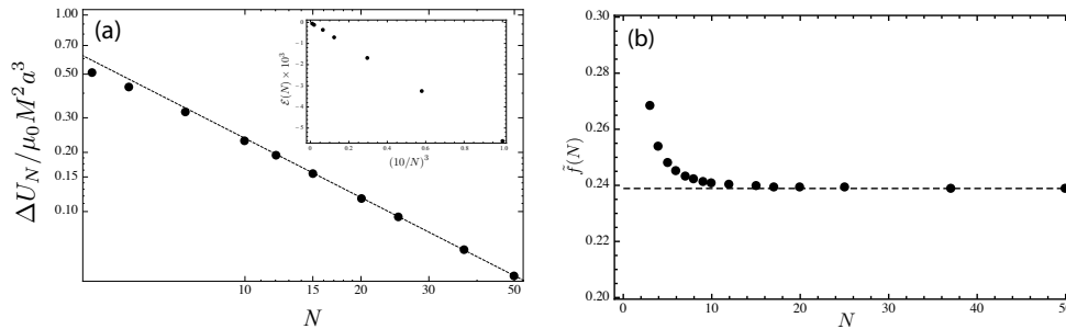
Figure 4. Numerical and asymptotic results for the effective bending stiffness. (a) The numerically computed change in energy \Delta U_N as a function of N (points) rapidly tends to the asymptotic result (2.24) (dashed line). Although the error estimate in (2.24) leads us to expect that \mathcal{E}(N) \sim N^{-2} , numerical computations reveals that in fact \mathcal{E}(N) \sim N^{-3} (see inset). (b) The behaviour of the dimensionless bending stiffness \tilde{f}(N) = f(\sin \frac{\pi}{N}, N) , with f as defined in (1.2), computed numerically (points) and in the limit N \gg 1 (dashed line).
