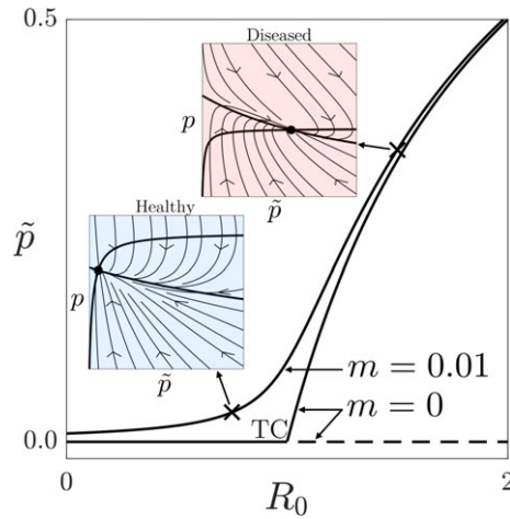
Figure 2. Bifurcation diagram for Prusiner's heterodimer model (2.1). Stable and unstable branches of equilibria are solid and dashed, respectively (only non-negative branches are shown). 'TC' marks a transcritical bifurcation point. Insets: Phase portraits of healthy (blue) and diseased (red) dynamics at R_0 = 0.75 and R_0 = 1.5 , respectively, showing the unique positive equilibrium at the intersection of the system's nullclines.
